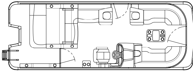
CATALINA/CASCADE 2385 VERSATILE REAR BENCH
