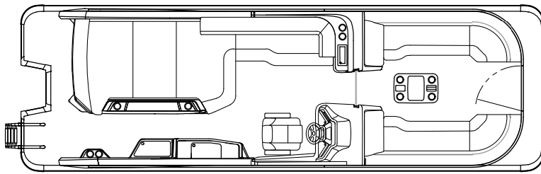
CATALINA/CASCADE 2785 VRB WINDSHIELD
