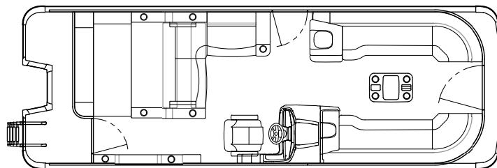
CATALINA/CASCADE 2585 VERSATILE REAR LOUNGER
