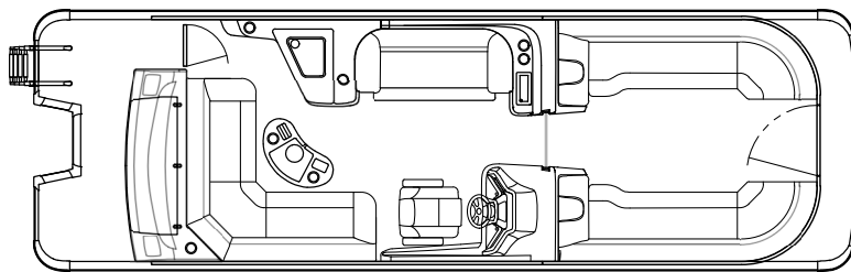
CATALINA/CASCADE 2785 ELITE WINDSHIELD
